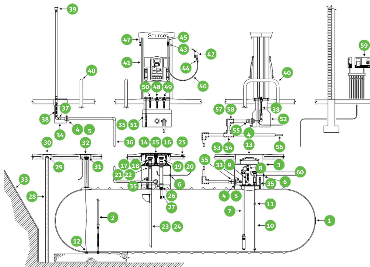
Figure 6. Typical station fuel dispenser and underground storage piping.
